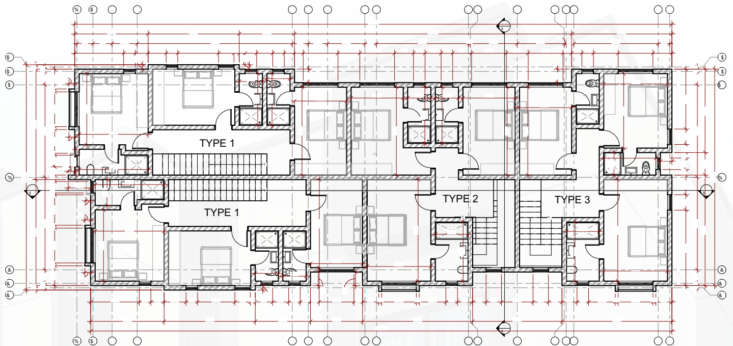
FIRST FLOOR
